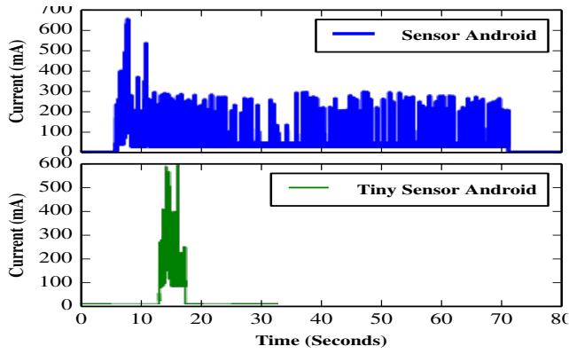
Figure 2: Current draw for a single sense-and-send cycle. Flaws in both approaches are visible. Tiny Sensor Android sleeps at a high 8 mA, whereas Sensor Android does not return to sleep for almost one minute.
