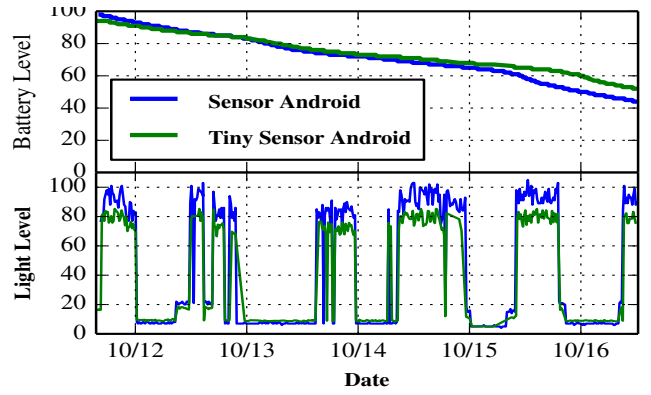
Figure 1: Lifetime results for two light sensing applications. Both approaches could achieve an 8–9 day lifetime.
